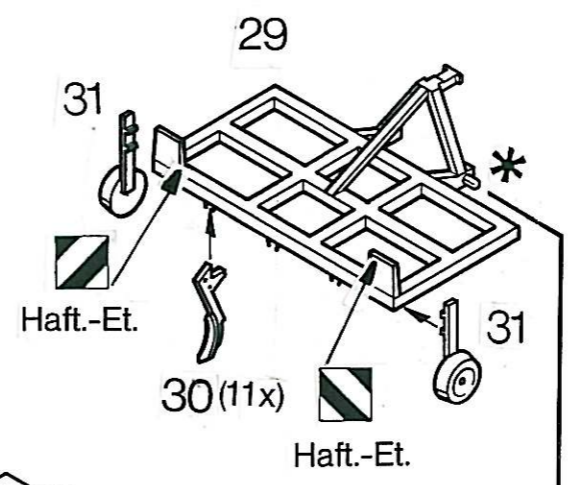
Frontgrubber Front mounting chisel Chisel attelage avant
